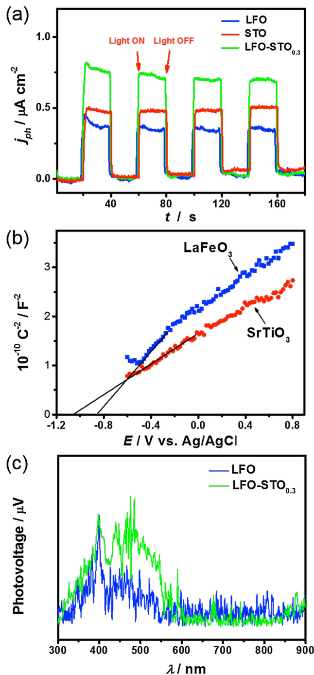
Fig. 5. (a) Transient photocurrent responses of the as-prepared STO, LFO and LFO- \text{STO}_{0.3} composite photoanodes, recorded at potential of 0.2 V vs. Ag/AgCl in 0.1 M \text{Na}_2\text{SO}_4 aqueous solution under visible light irradiation ( \lambda = 420 nm); (b) Mott-Schottky plots of the \text{LaFeO}_3 and \text{SrTiO}_3 electrodes in 0.1 M \text{Na}_2\text{SO}_4 at the frequency of 1000 Hz and DC potential range of -0.6 to +0.8 V vs. Ag/AgCl, perturbation bias: 5 mV; (c) SPS spectra of the pristine \text{LaFeO}_3 and LFO- \text{STO}_{0.3} composite.
