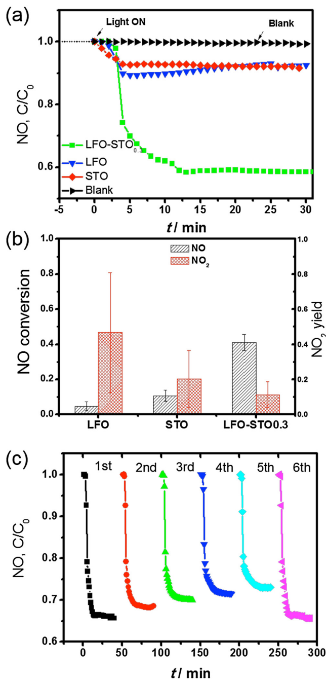
Fig. 4. (a) NO photocatalytic removal profile C/C_0 as a function of time over the as-prepared LFO, STO and LFO- \text{STO}_{0.3} composite; (b) Comparison of the NO conversion rate ( C/C_0 ) and \text{NO}_2 yield over the as-prepared LFO, STO and LFO- \text{STO}_{0.3} composite; (c) Cyclic NO degradation tests with the LFO- \text{STO}_{0.3} composite under visible light irradiation ( \lambda \geq 420 nm).
